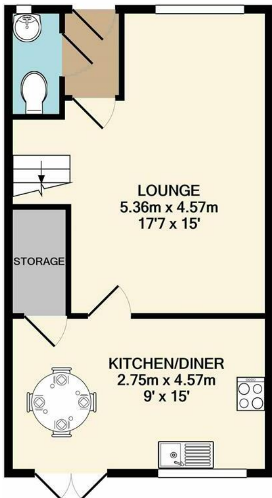
GROUND FLOOR APPROX. FLOOR AREA 37.1 SQ.M. (399 SQ.FT.)
